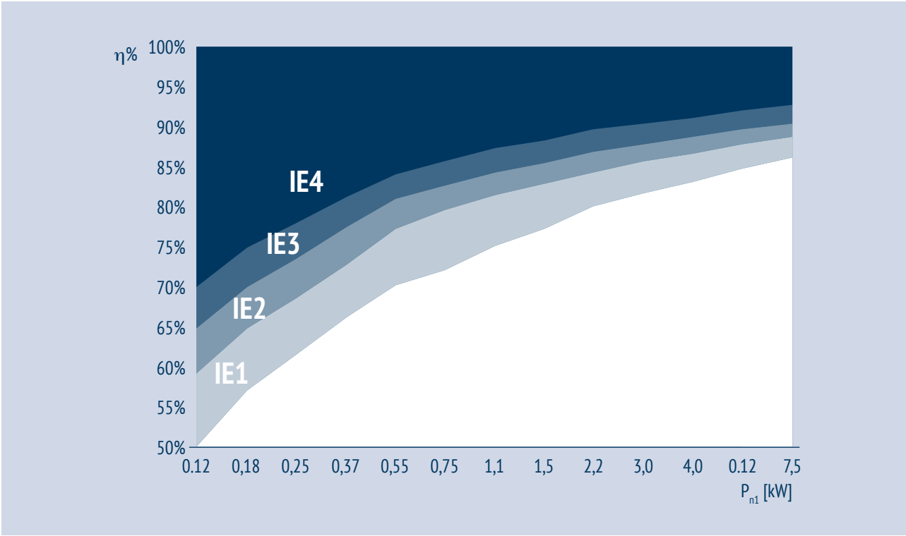
IE efficiency classes for 4-pole motors at 50 Hz
