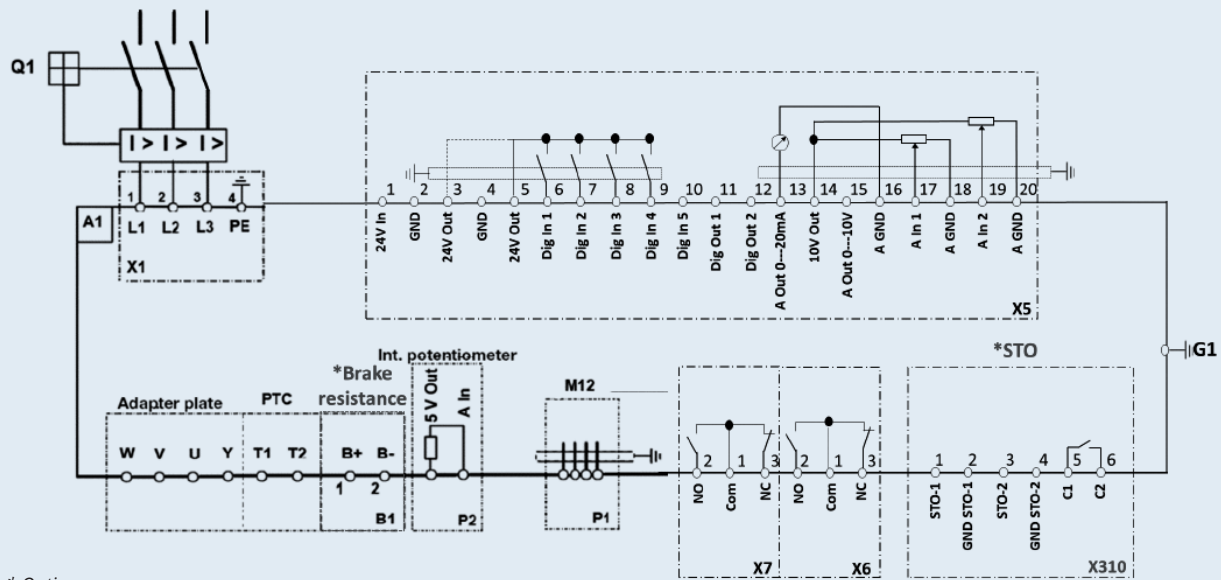
Example of DGM version wiring
