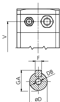
SHAFT END SECTION
