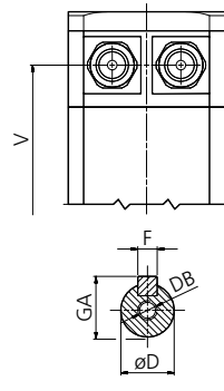
SHAFT END SECTION
